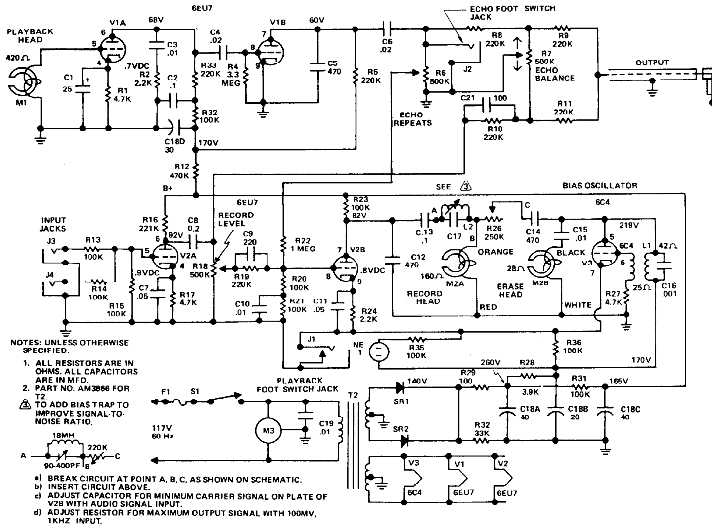
ECHOPLEX EP-2 SCHEMATIC DIAGRAM - SERIAL NO. 5500 TO 5938
