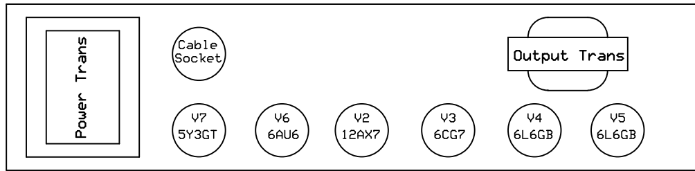
Tube Location Chart - Lower Chassis V1 Located on Pre-amp Chassis
