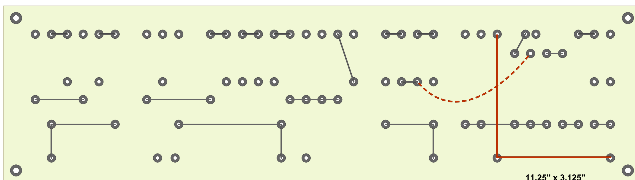
Hoffman Plexi 6V6 Turret Jumper Guide
