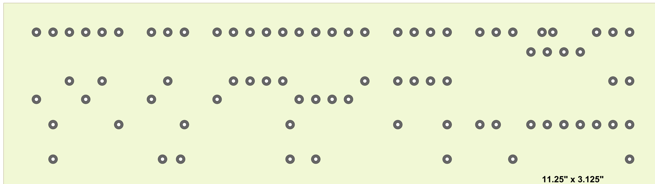
Hoffman Plexi 6V6 Drill Guide (80 Turrets)
