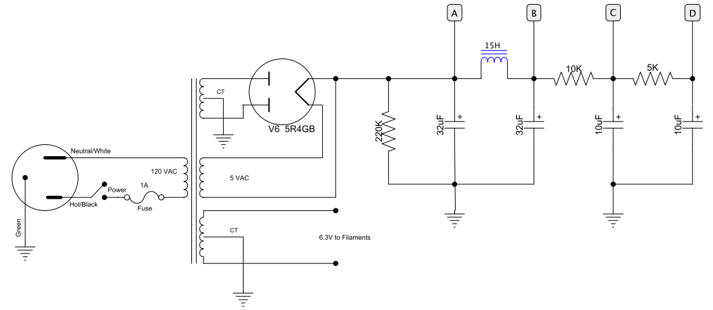
18 Watt Plexi Reverb MV
