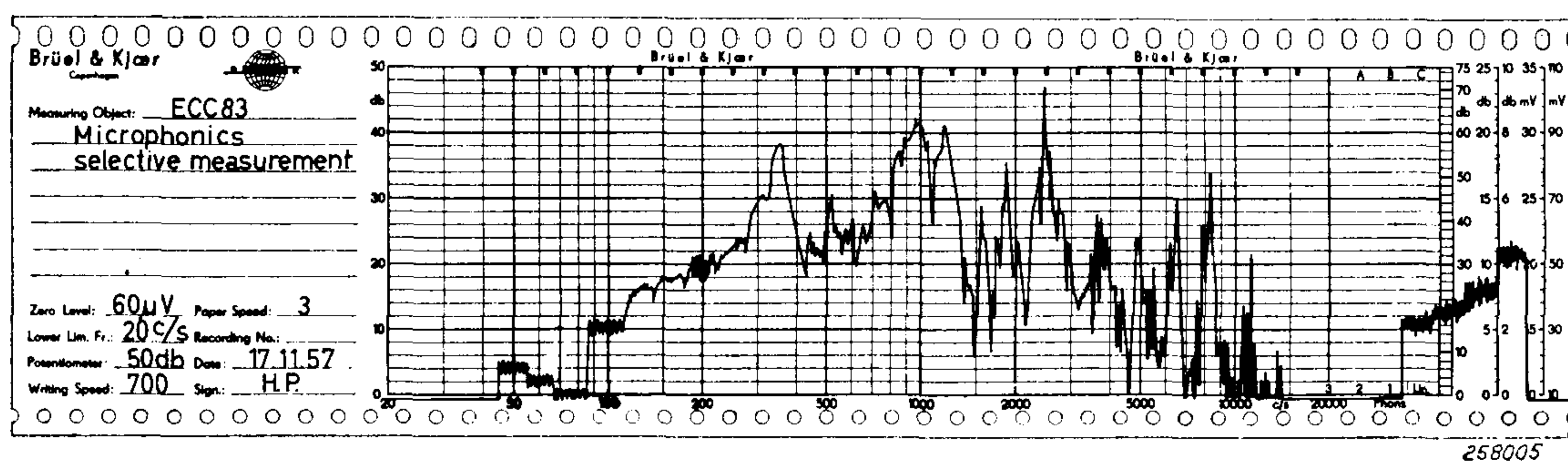
Fig. 7. Selective measurement of the microphonics from a tube type ECC 83.
