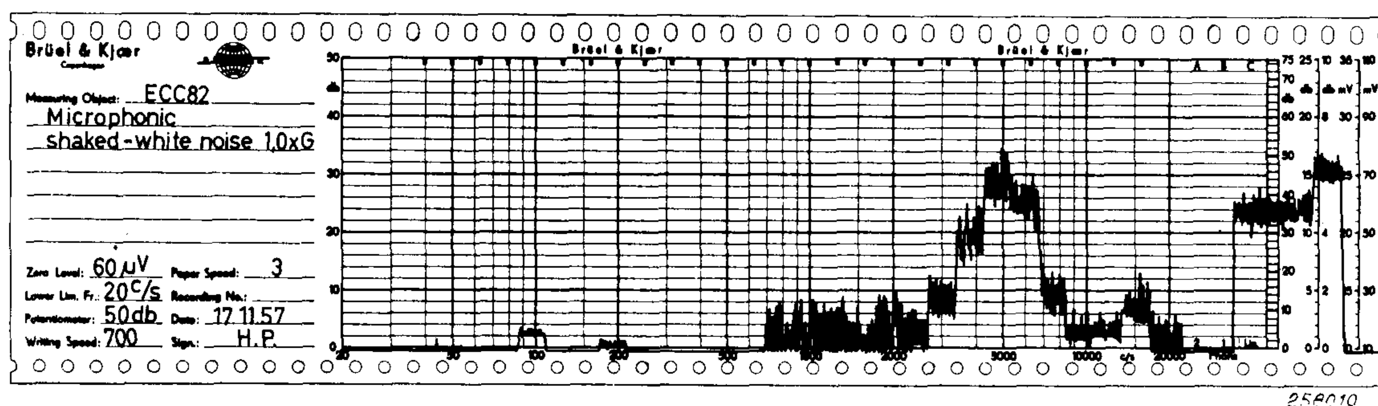
Fig. 10. Frequency analysis of the microphonics from a tube type ECC 82 shaken by means of a vibrator energised from a white noise generator. (Random motion method).
