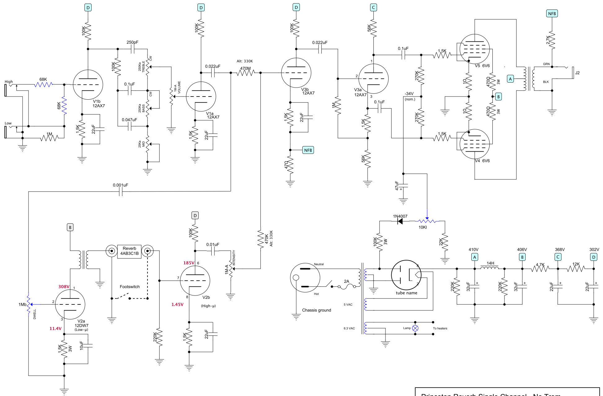
Princeton Reverb Single Channel - No Trem One-tube 12DW7 Reverb after tubenit Date: 02/11/2025 Rev. 1.3
