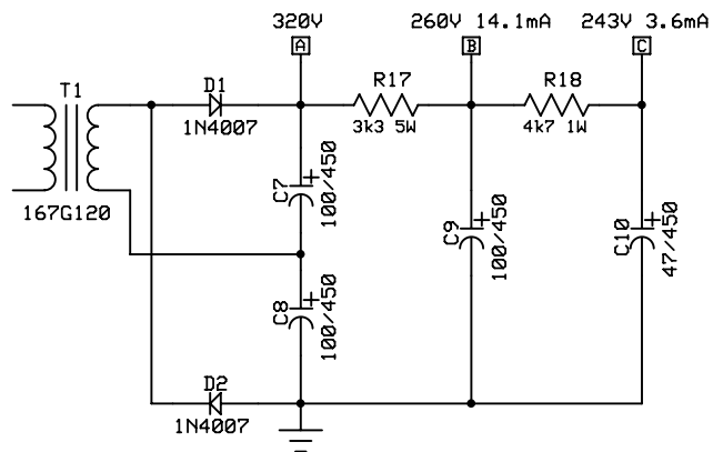
B+ power supply estimated for 2 channels
