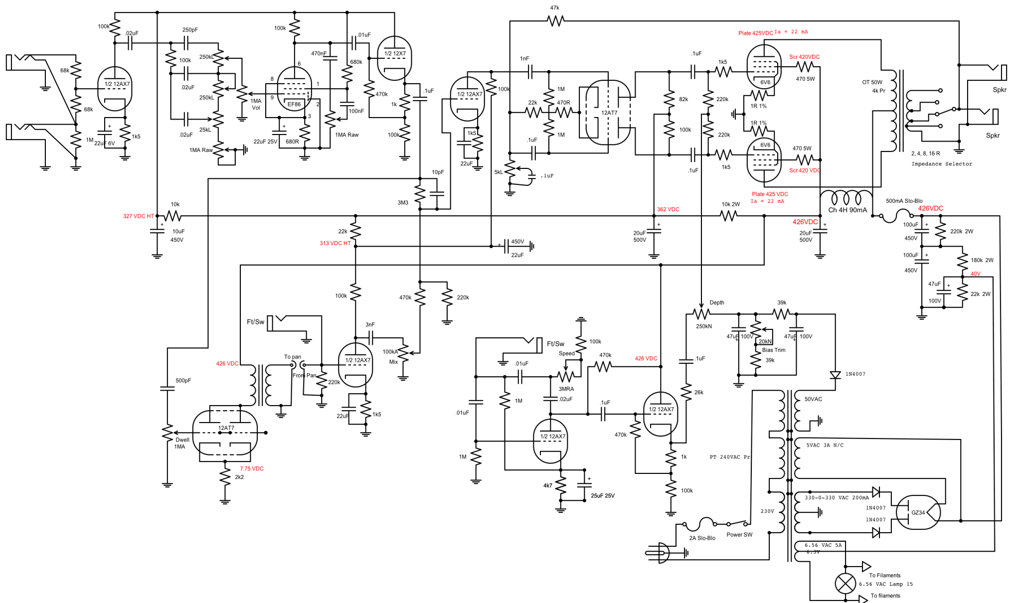
"BFDR++ with EF86" Trem with AC-coupled CF tubeswell Ver 4 1/09/10 Page #
