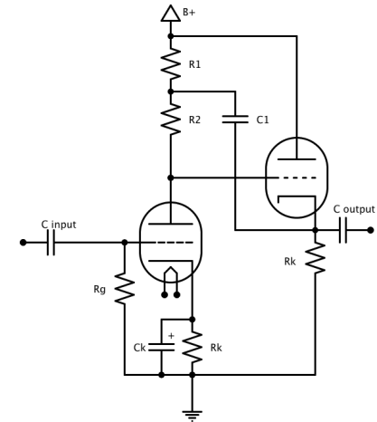
DC-coupled Bootstrapped for increased gain
