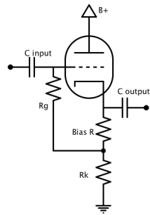
AC-coupled Bootstrapped for increased input impedance
