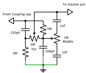
Alternate Tone Stack (using 1M pots)
