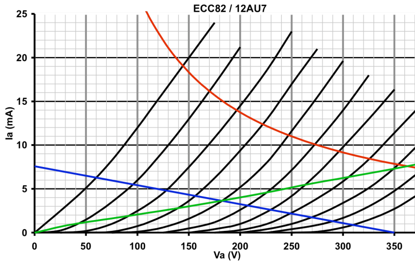
2 x 22k resistors (44k load) 2k2 bias resistor (-8V)
