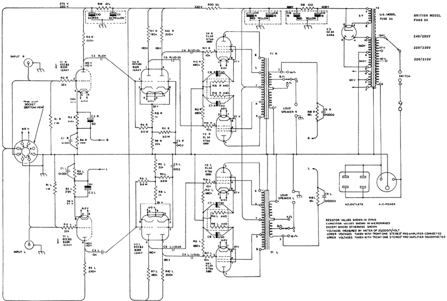
CIRCUIT DIAGRAM
