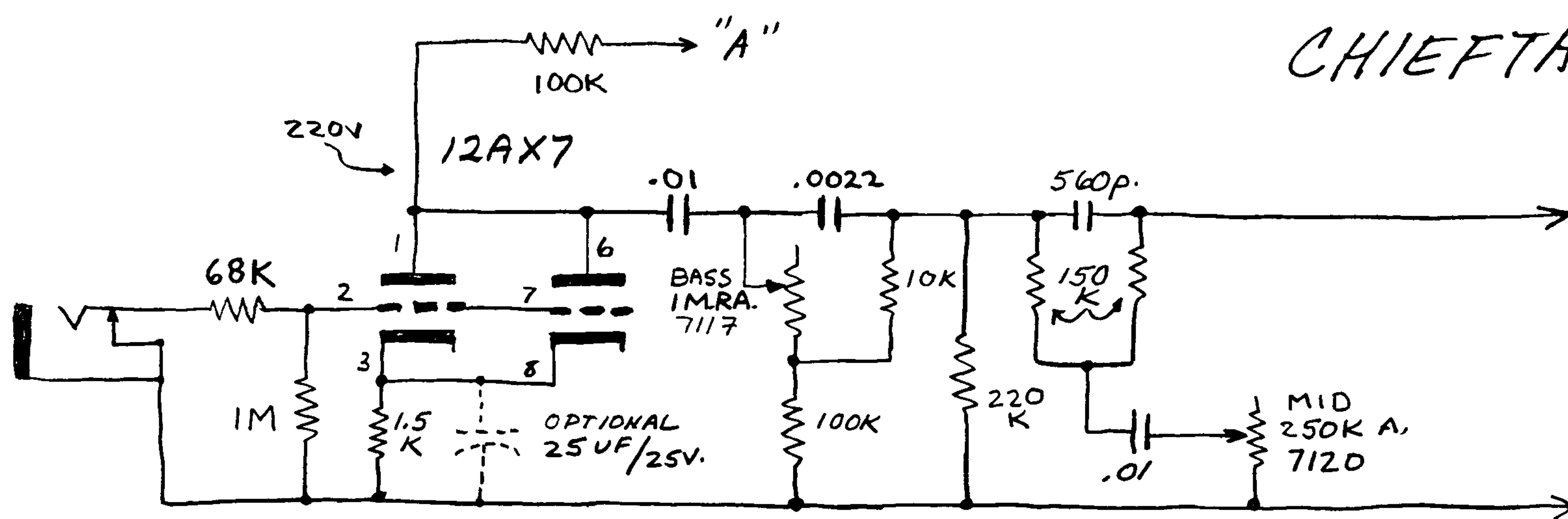
FIRST STAGE PREAMP
