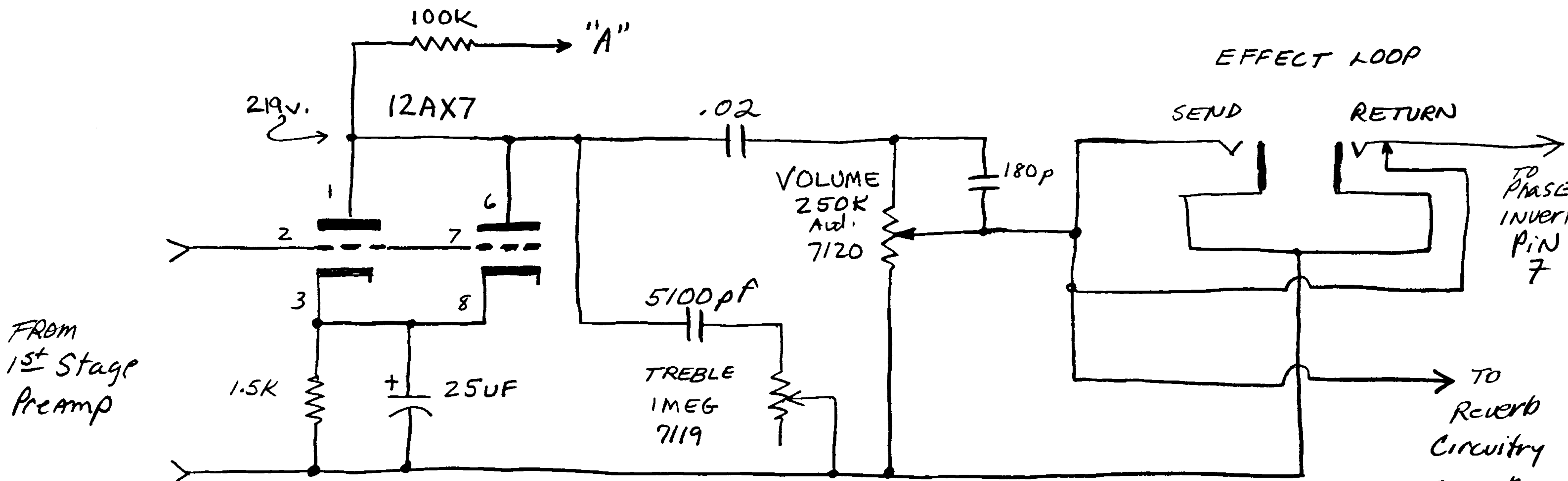
SECOND STAGE Preamp
