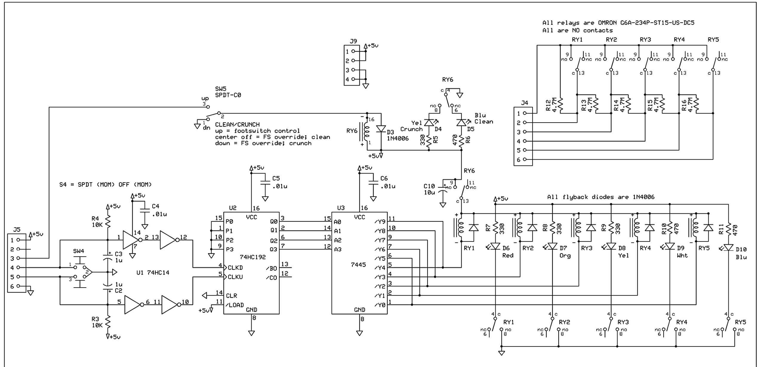
Control Board
