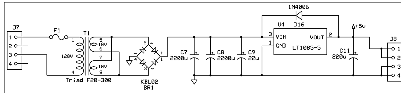
Power Supply Board
