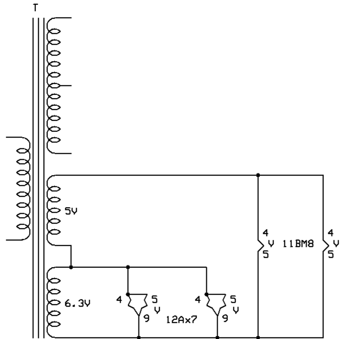
Hammond-270CAX
