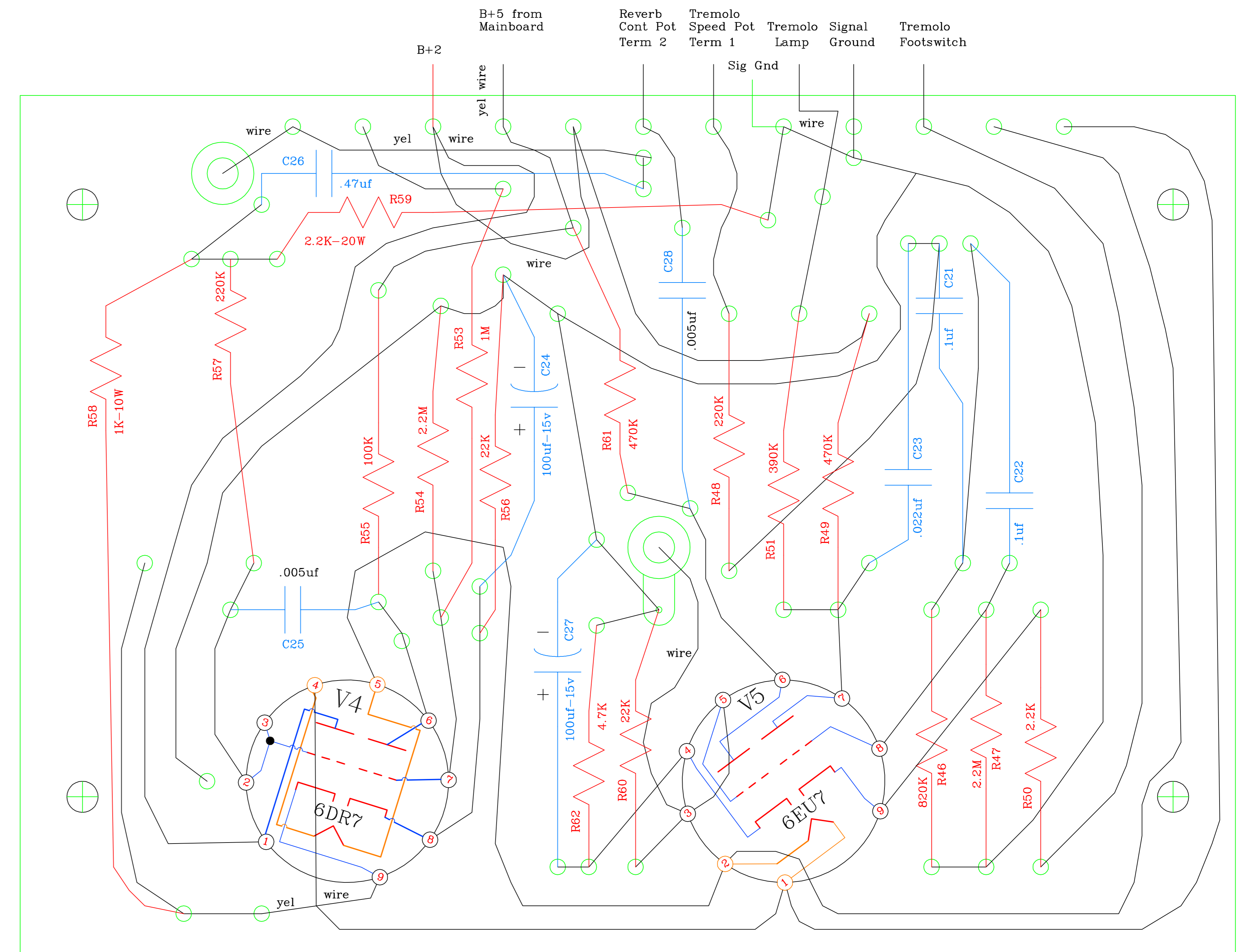
Reverb / Tremolo Board
