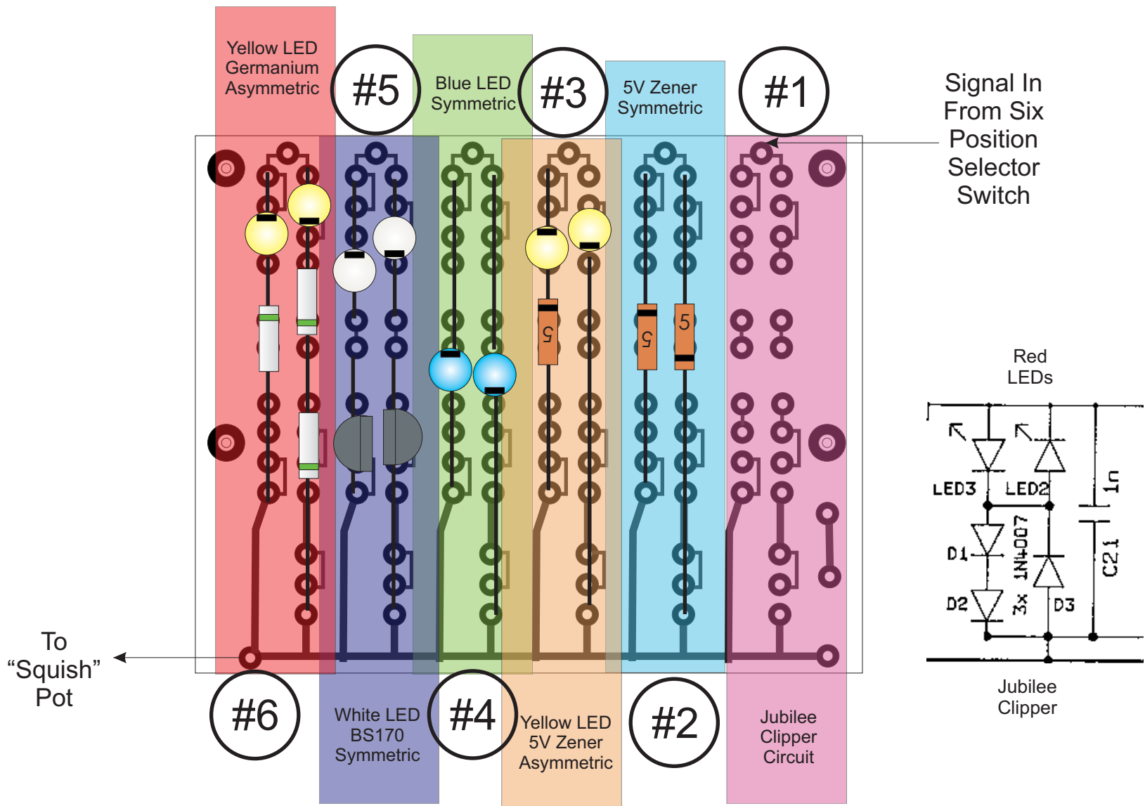
JCM-800 Clipping Circuit Array
