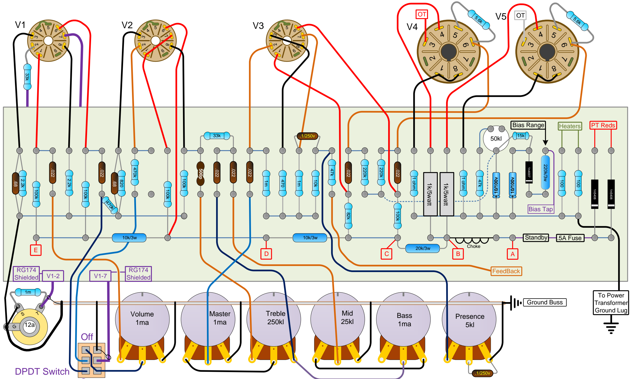
Hoffman Amplifiers Plexi50 – with Hot Switch Gain Mod
