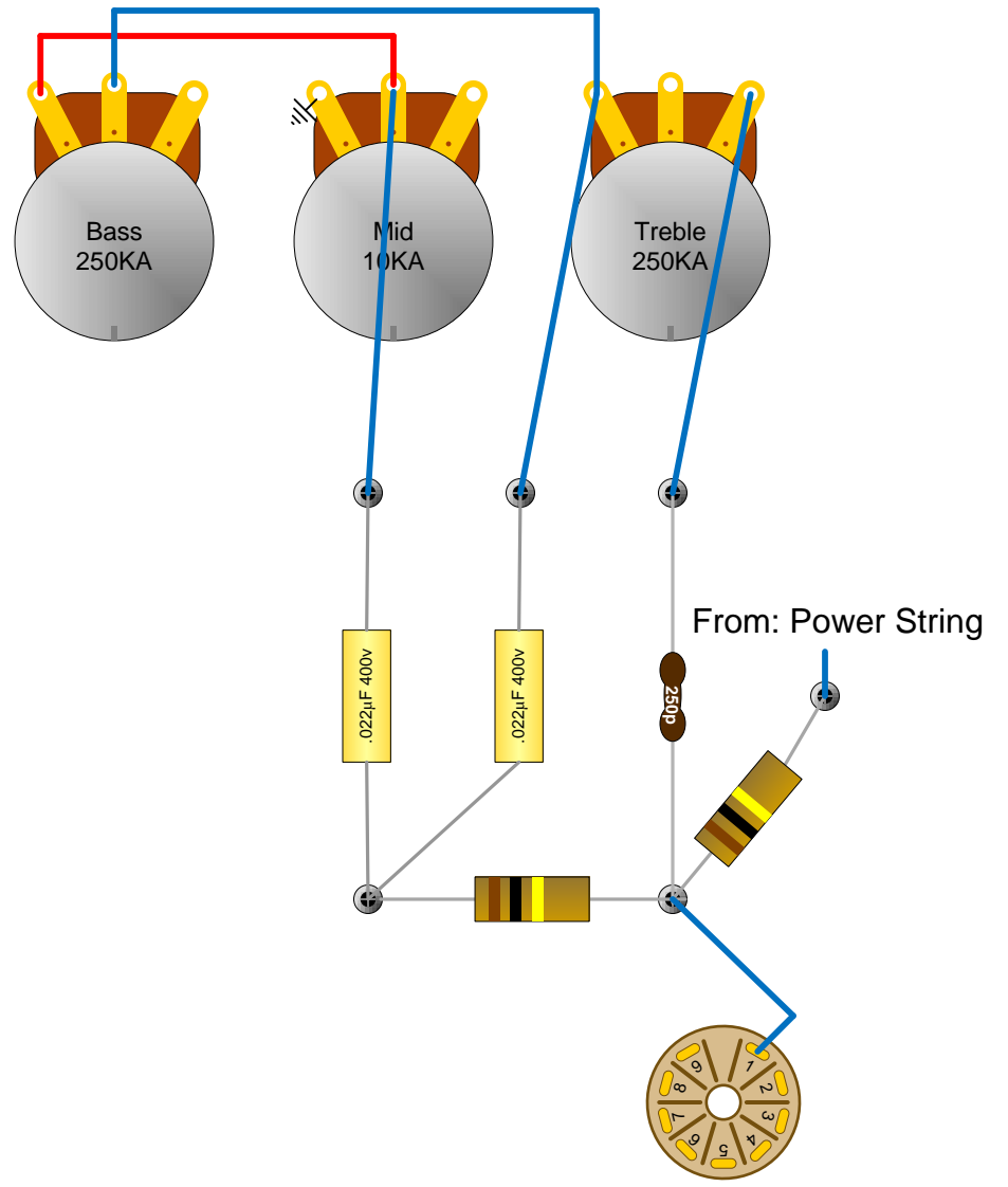
AB763 Blackface Tone Stack
