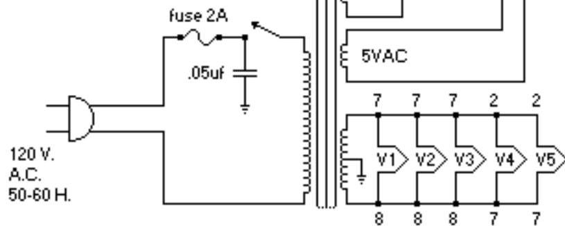
Ampeg Amplifier Model M-15 (6L6 version) Drawn By: Joe Piazza 5/7/97
