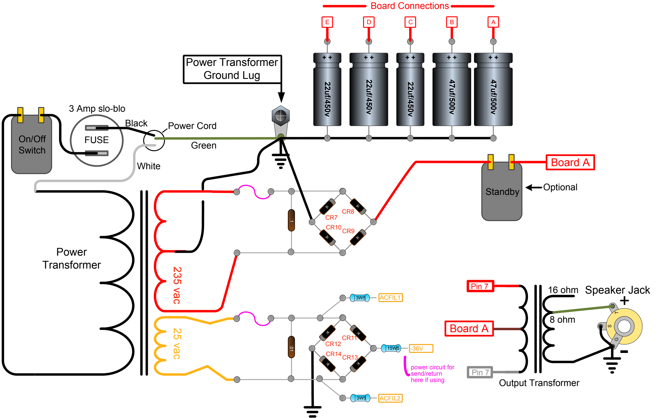
Peavey Classic 30 Conversion to Hoffman Amplifiers AC30
