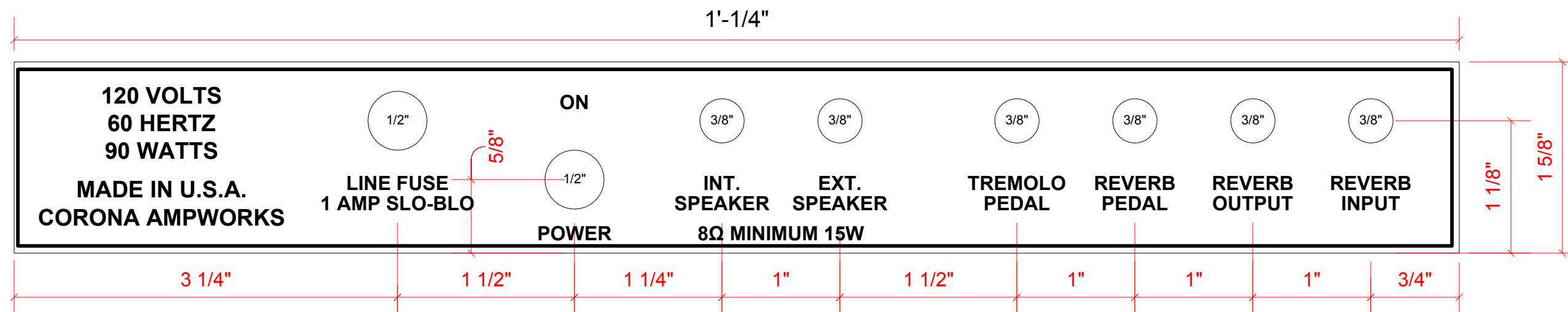
Back plate
