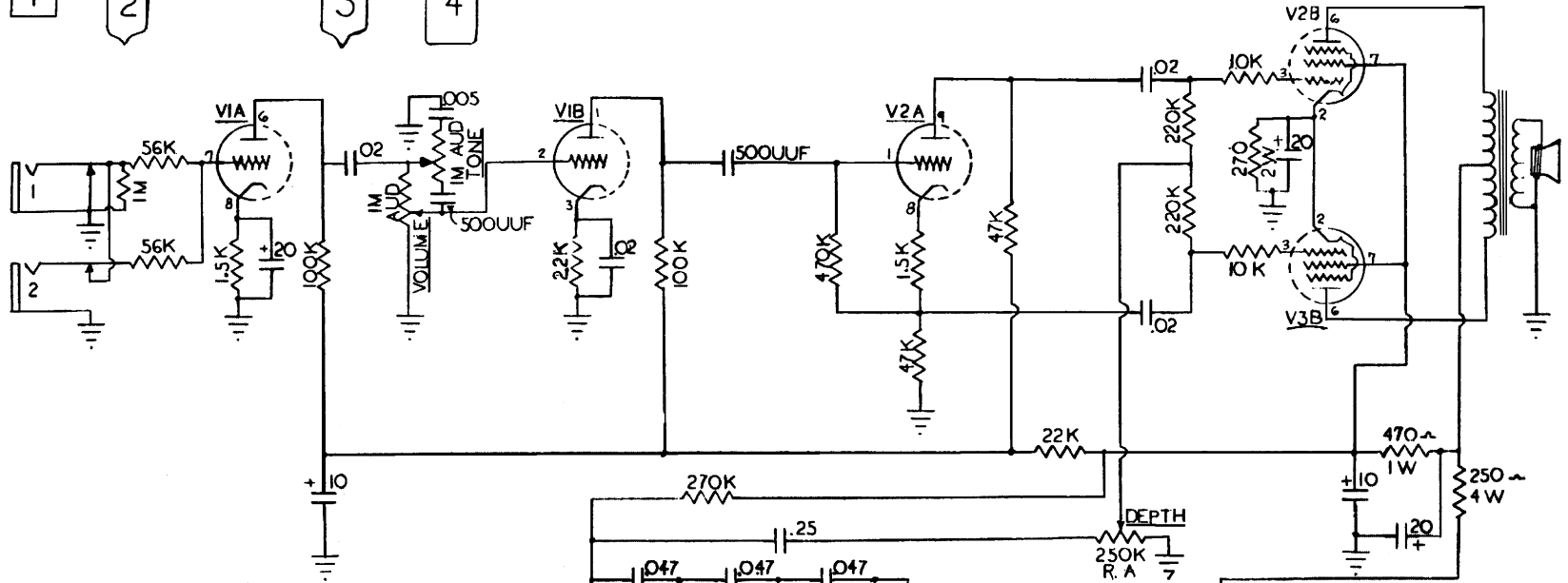
VOLTAGE CHART *
