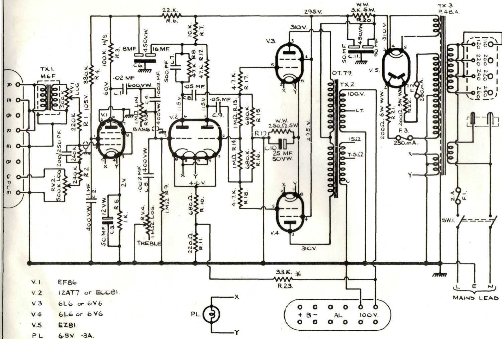
TITLE CIRCUIT DIAGRAM, 15 WATT AMPLIFIER TYPE 562/1/D.
