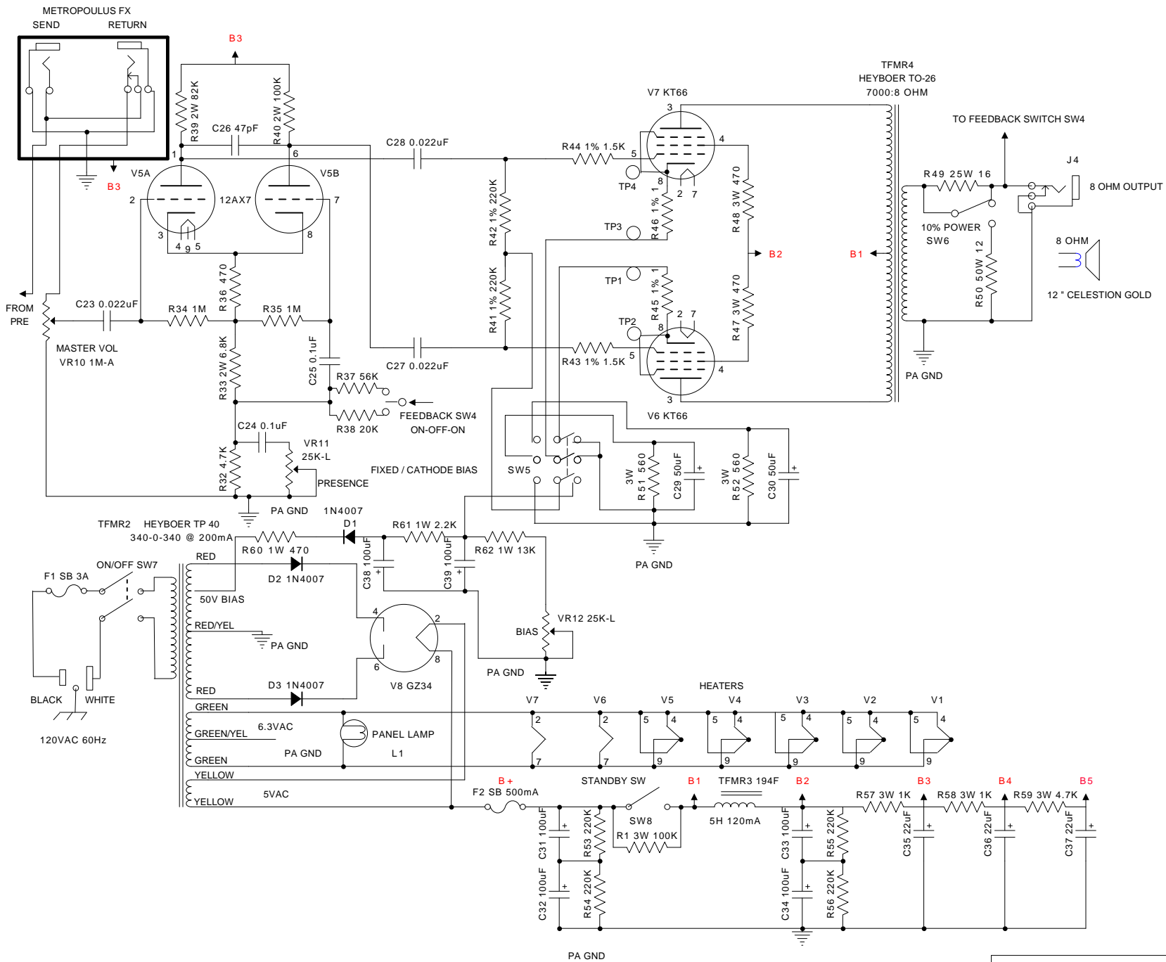
TREMOR-VERB SL2DRR FX, MV, PI, POWER AMP, AND POWER SUPPLY SWAMPERTECH AMPLIFIERS RED HILL, ALABAMA 4 SEPTEMBER, 2019
