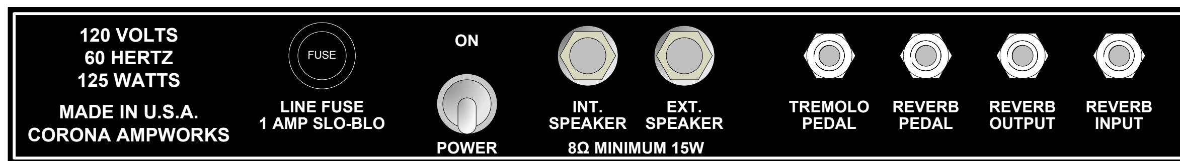
Back plate
