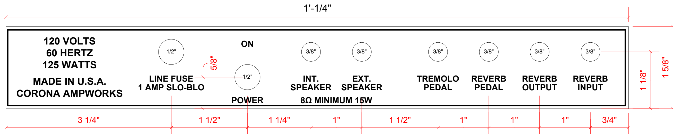
Back plate
