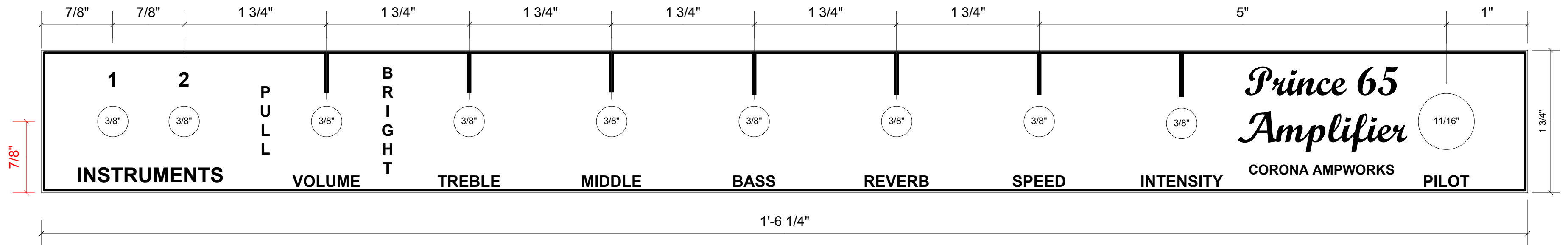
Front plate
