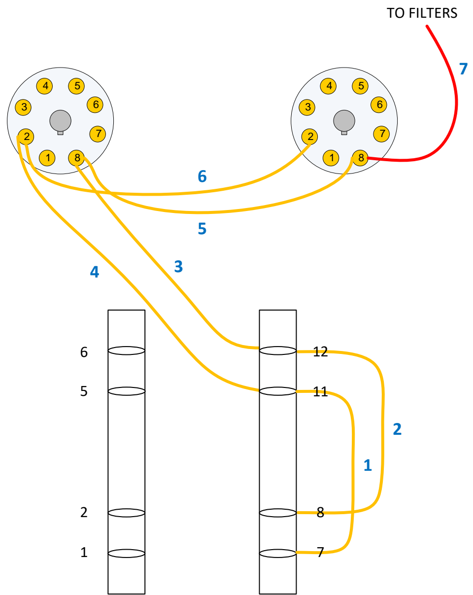
185D10 Parallel
