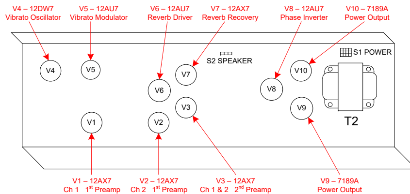
TUBE LOCATOR
