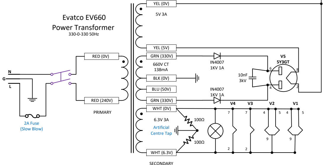
Fender Deluxe 5E3 Clone All resistors 1W unless stated
