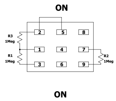
TPDT Switch
