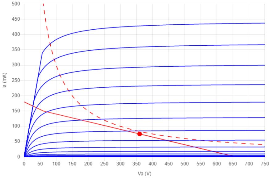
Anode Characteristic Graph: KT66 - www.vtadiy.com
