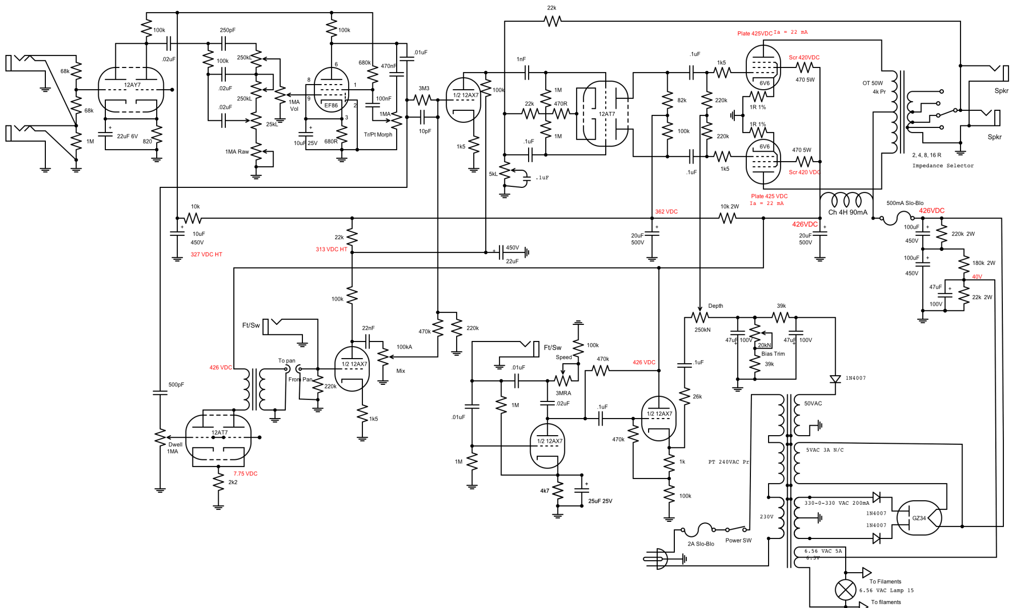
"BFDR+ with EF86 variant" Trem with AC-coupled CF tubeswell Ver 4 1/09/10 Page #
